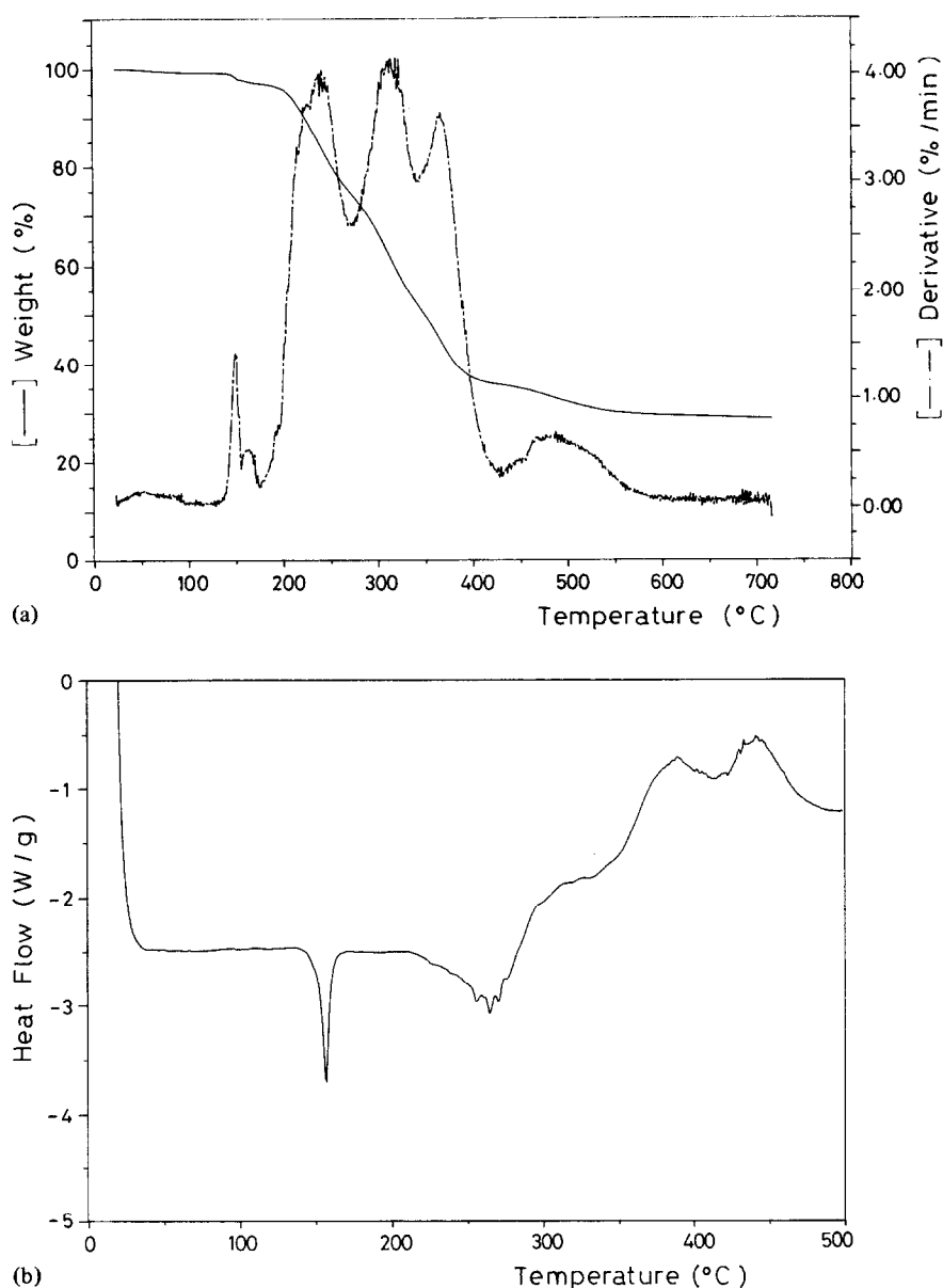
Fig. 1. \text{Mo}_2(\text{CO})_{10}[\mu\text{-Ph}_2\text{P}(\text{CH}_2)_4\text{PPh}_2] : (a) TG curve, (b) DSC curve.
