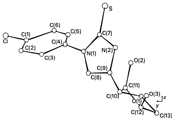
Fig. 1. Molecular conformation.
