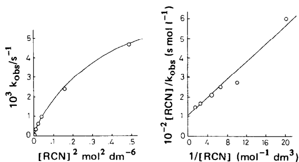
Fig. 1. Reaction of 1,3,5-trimethylbenzonitrile with [(\eta^6\text{-C}_7\text{H}_8)\text{Mo}(\text{CO})_3] in dichloroethane at 30.0 °C. (a) Plot of k obs versus [RCN] 2 , (b) plot of [RCN]/ k obs versus 1/[RCN].
