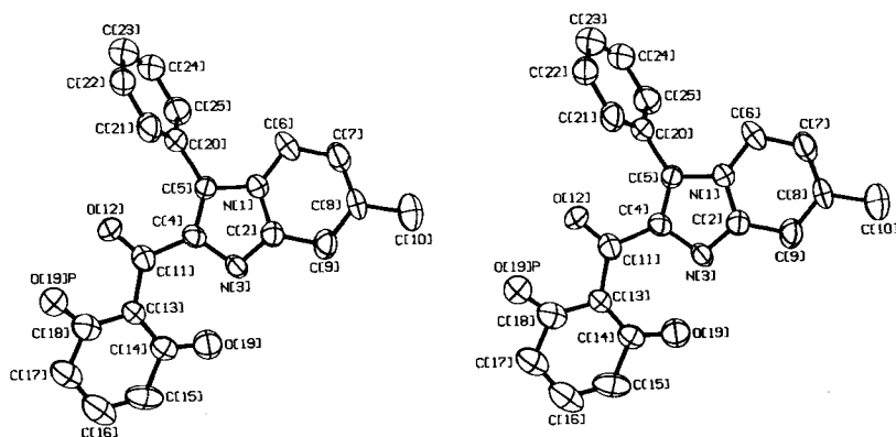
FIGURE 2. X-Ray crystal structure of 2- o -hydroxybenzoyl-7-methyl-3-phenylimidazo[1,2- a ]pyridine.
