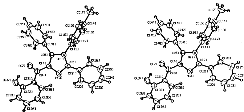
FIGURE 1. X-Ray crystal structure of 4- o -hydroxybenzoyl-2,5-diphenyl-1- p -tolylimidazole ( 6b ).
