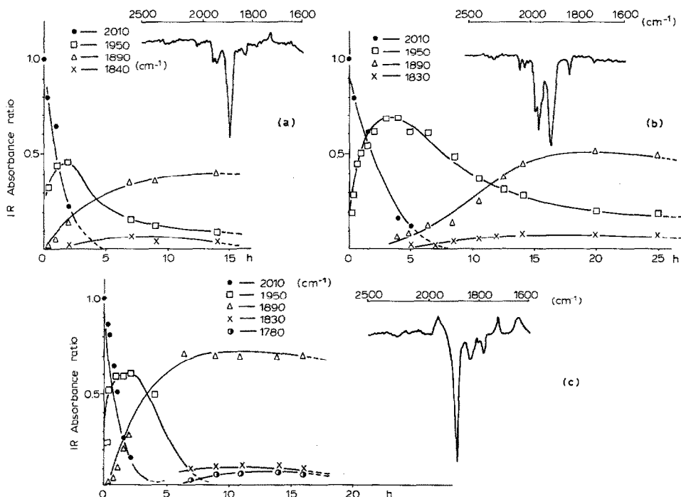
Fig. 5. Photochemistry of Mn 2 (CO) 10 with tri-n-butylphosphine (a): T 250 K under N 2 ; (b): T 250 K under CO; (c): T 297 K under N 2 . (IR absorbance ratios were calculated with the Mn 2 (CO) 10 absorbance as reference.)
