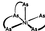
Figure 1. A diagrammatic drawing of the coordination polyhedron in [\text{Ni}(\text{diars})(\text{triars})](\text{ClO}_4)_2 . Crystals are monoclinic, space group \text{P2}_1/\text{c} ; a = 18.41 , b = 20.21 , c = 12.61 Å, \beta = 125.80^\circ , Z = 4 formula units per unit cell. At the present stage of least-squares refinement, the residual R = 0.18 . The basal plane Ni-As distances are 2.26, 2.27, 2.30, and 2.32 Å. The apical Ni-As distance is 2.39 Å. The site below the square plane appears to be unoccupied.
