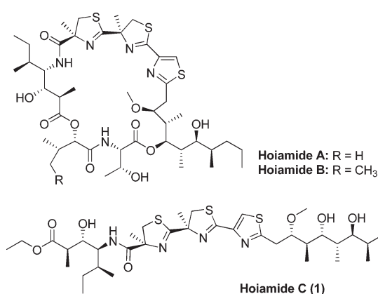
Figure 1. Structures of hoiamides A–C.
