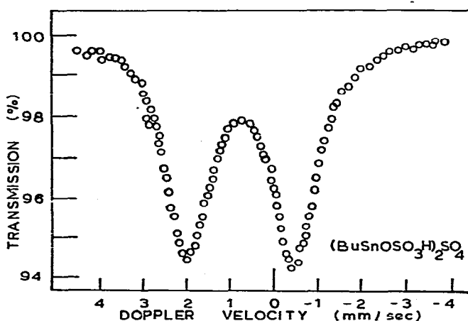
Fig. 1. Mössbauer spectrum of (\text{n-C}_4\text{H}_9\text{SnOSO}_3\text{H})_2\text{SO}_4 at 84^\circ\text{K} using a source of \text{BaSnO}_3 at room temperature. The isomer shift reference point is the center of a \text{BaSnO}_3 – \text{BaSnO}_3 resonance spectrum at 294^\circ\text{K} .
