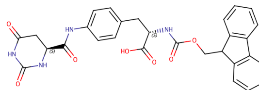
Fmoc-L-Aph(L-Hor)-OH CAS#1253282-31-3
