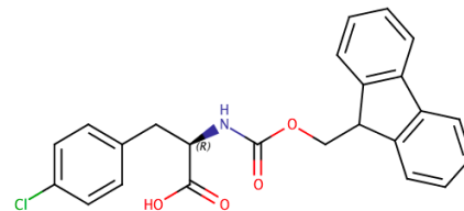
Fmoc-D-Phe(4-Cl)-OH CAS#142994-19-2
