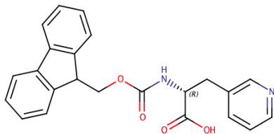
Fmoc-D-3-Pal-OH CAS#142994-45-4
