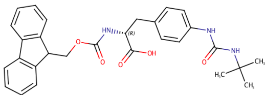
Fmoc-D-Aph(tBuCbm)-OH CAS#1433975-21-3
