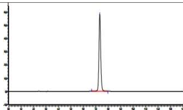
Figure 1:HPLC-DAD chromatogram of U-[ 13 C 7 ]-Patulin
