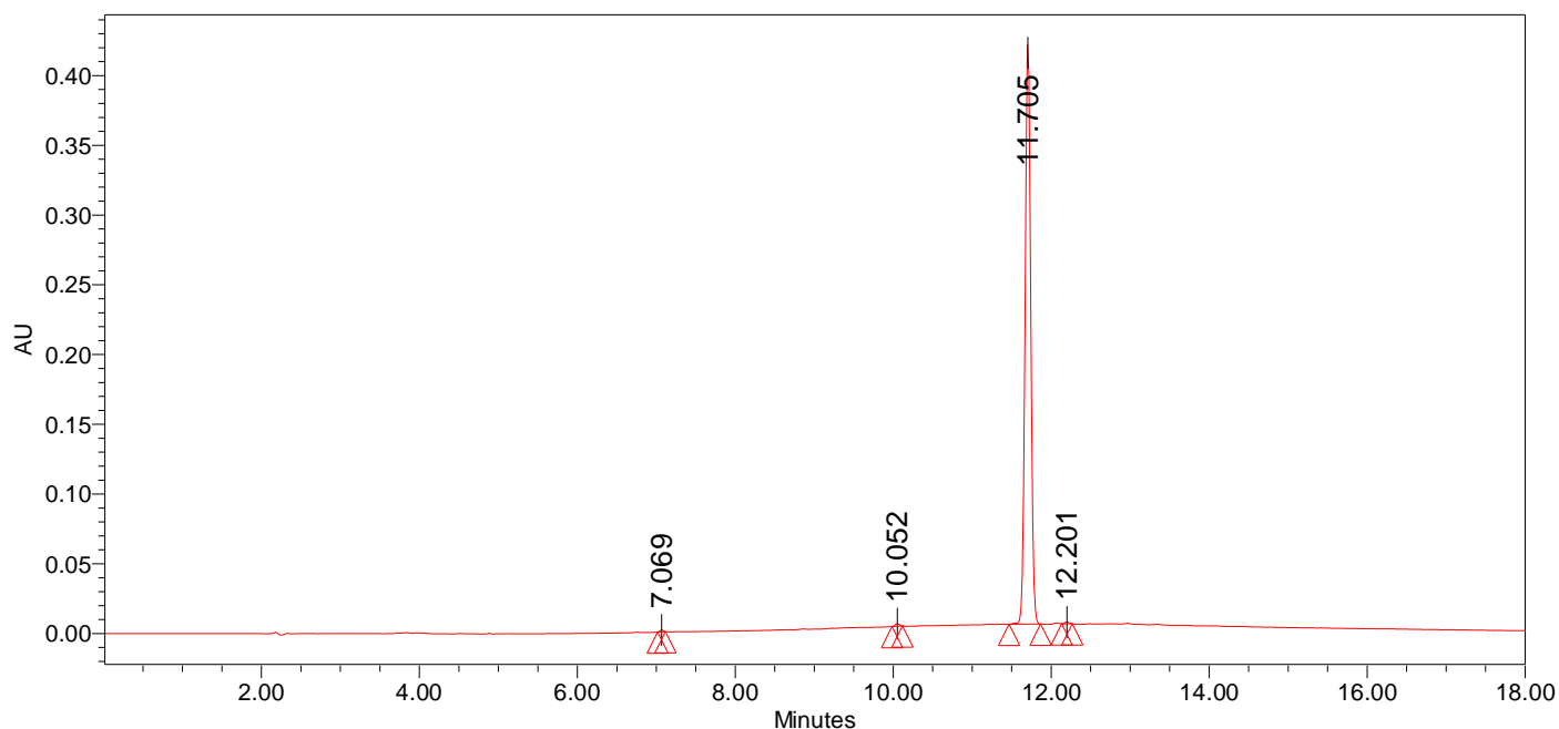
235nm Chromatogram
