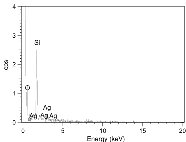
Fig. 4 EDX spectrum of silver embedded silica particles
