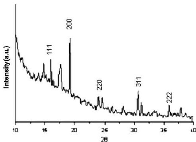
Fig. 2 The XRD pattern of the NiO nanoparticles prepared at 100 °C to native defects such as Ni interstitials and O vacancies as suggested by Lyu et al. [18].
