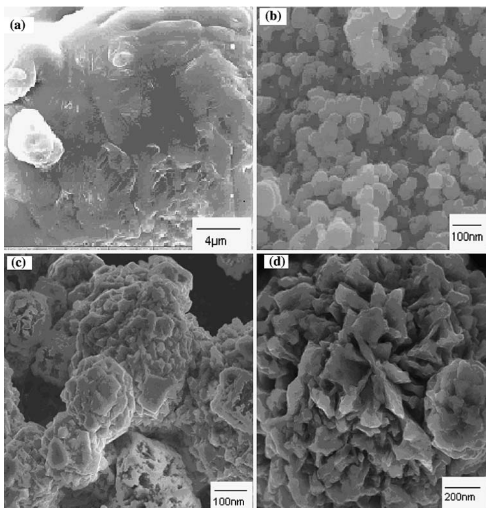
Fig. 1 FESEM images of nanoparticles and nanoflowers obtained by the reaction of nickel metal with water at 100 °C for 12–36 h. (a) Images of samples at room temperature for 12 h, (b) at 100 °C for 12 h, (c) at 100 °C for 24 h, (d) 100 °C for 36 h
