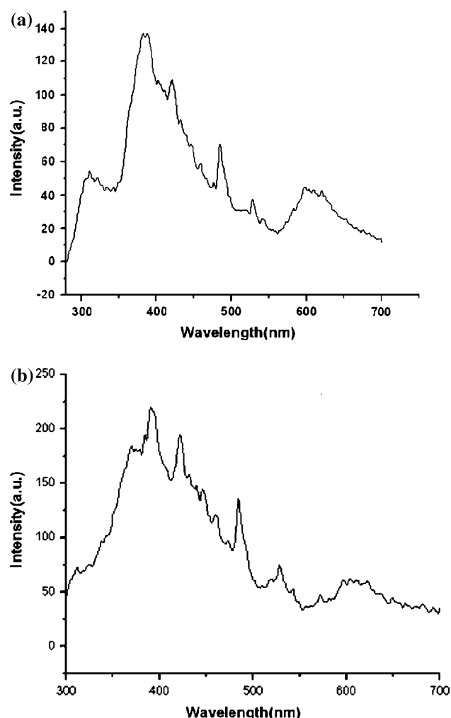
Fig. 3 (a) Room temperature photoluminance spectra NiO nanoparticles prepared at 100 °C. (b) Room temperature photoluminance spectra of NiO nanoflowers prepared at 100 °C
