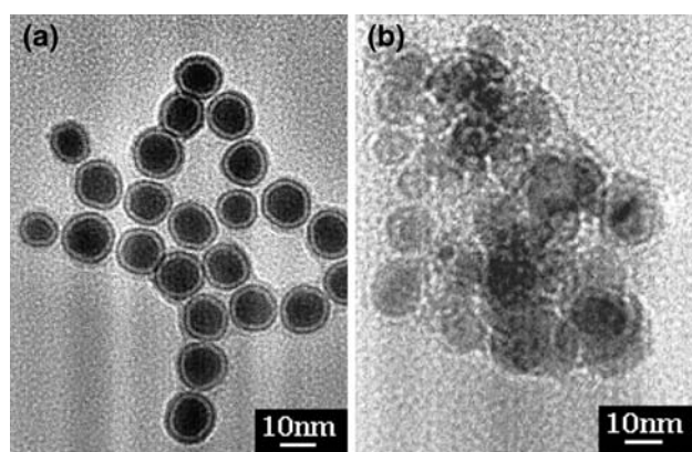
Fig. 2 TEM image of \varepsilon -Fe 3 N nanoparticles. (a) Coated with surfactant, (b) without any surfactant
