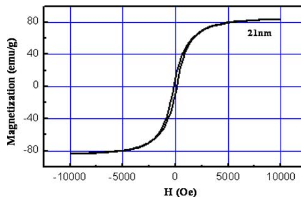
Fig. 5 Hysteresis loops at room temperature of the \epsilon -Fe 3 N nanoparticles under the field up to 10 kOe ( \sigma_s = 83.5 emu/g)
