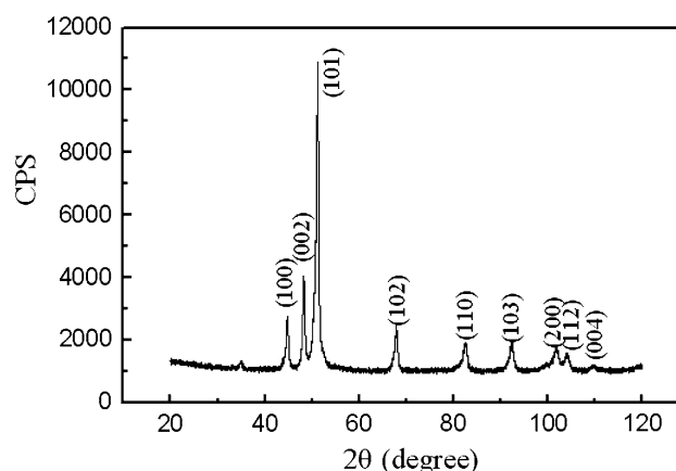
Fig. 1 X-ray diffraction pattern of \epsilon -Fe 3 N magnetic particle (Co K \alpha 1 )
