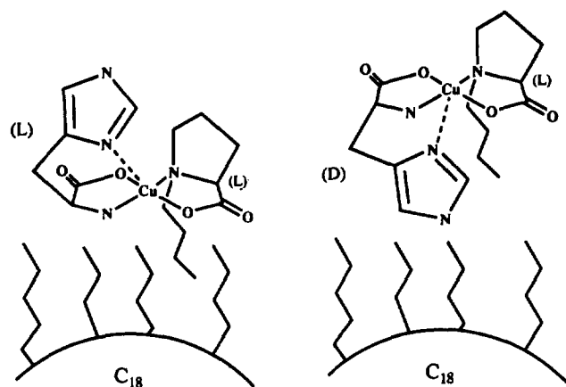
Figure 4. Interaction of the ternary complex containing N-alkyl-L-proline and D- (or L-) His with the alkyl chain of C_{18} column.
