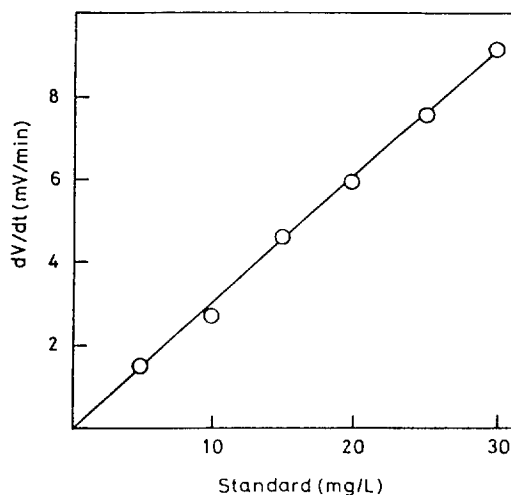
Figure 2. Relationship of the dV/dt and the concentration of glucose and glutamic acid.
