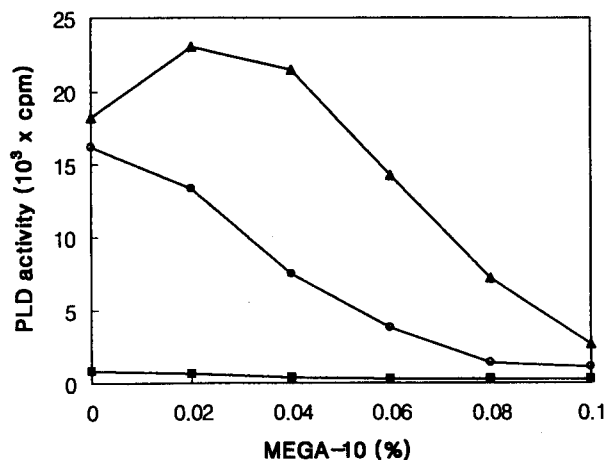
Figure 2. Effect of MEGA-10 concentration on microsomal PLD activity in the presence of varying amount of oleate. The assay mixtures maintained constant ionic strength with 375 mM NaCl. -■-, 2 mM; -○-, 5 mM; -▲-, 8 mM.
