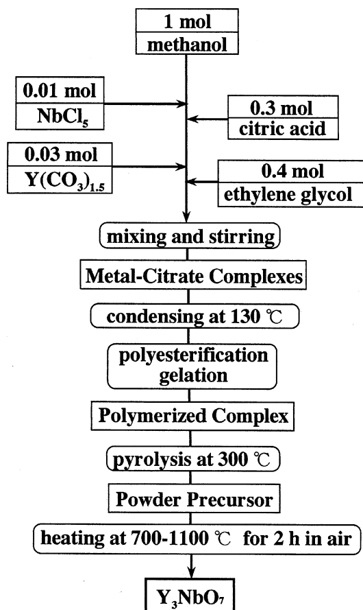
Figure 1. Flow chart for preparing \text{Y}_3\text{NbO}_7 by a modified Pechini-type polymerizable complex method.
