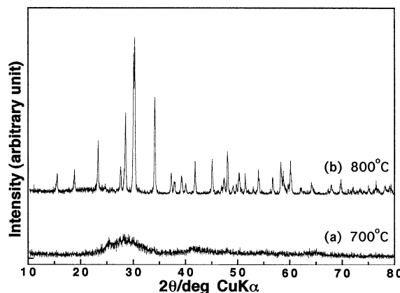
Figure 2. XRD patterns of the products obtained after calcining the powder precursor for \text{BaTi}_4\text{O}_9 in air for 2 h at (a) 700 and (b) 800 °C.
