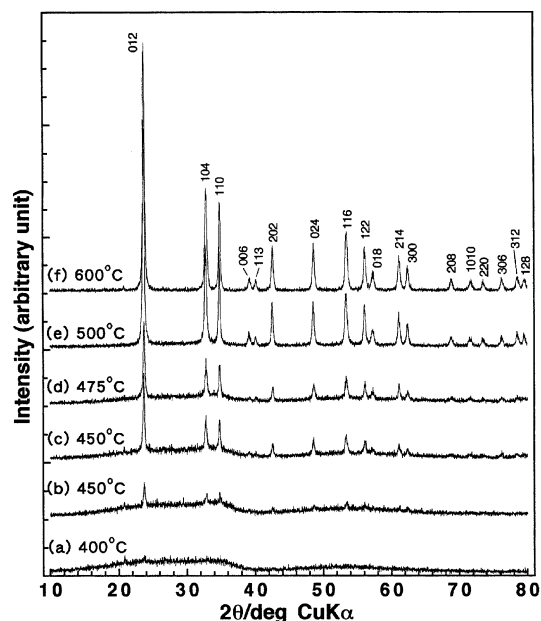
Figure 4. XRD patterns of the products obtained after calcining the powder precursor for \text{LiTaO}_3 in air for 2 h at (a) 400, (b) 450, (d) 475, (e) 500 and (f) 600 °C, and for 8 h at (c) 450 °C.
