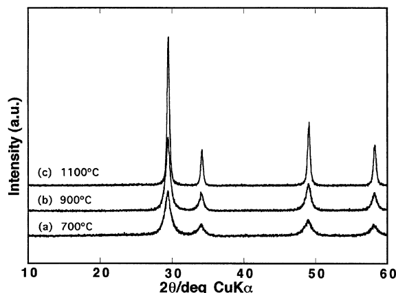
Figure 3. XRD patterns of the products obtained after calcining the powder precursor for \text{Y}_3\text{NbO}_7 in air for 2 h at (a) 700, (b) 900 and (c) 1100 °C.
