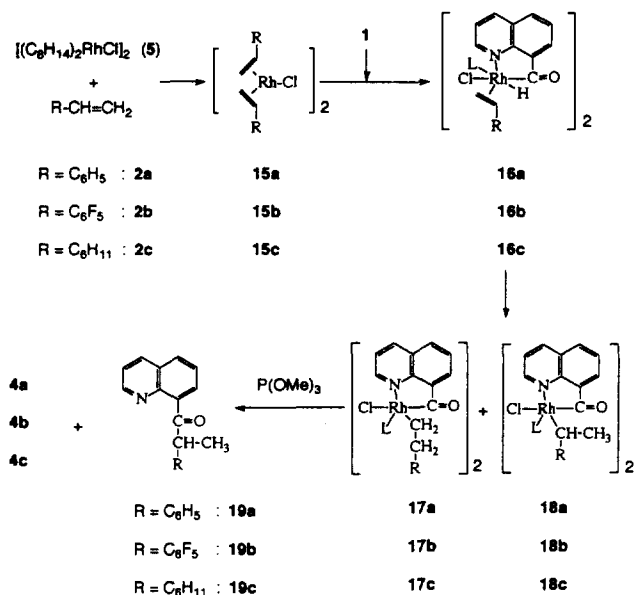
Scheme 3. Stoichiometric hydroacylation reaction of vinyl derivatives with 8-quinoline-carboxaldehyde (1) by 5 through hydrometallation and reductive elimination (L: CH 2 =CH-R).
