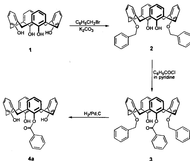
Scheme 1. Synthesis of monobenzoester calix[4]arene via di-benzoylation.
