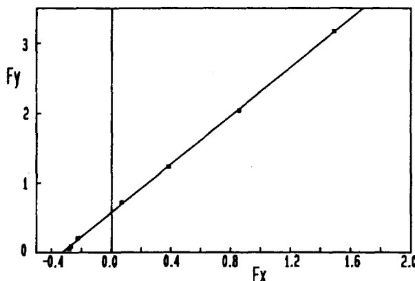
Figure 2. Determination of K_{1A} and K_{1B} for the 1:1 Cu(II)-Bistris system by eq. (2). F_x = \{(S - T_L + [\text{L}])[\text{H}^+]/(S + T_M - T_L + [\text{L}])\}10^7 . F_y = \{(T_M - S + T_L - [\text{L}])[\text{H}^+]^2/(T_M + S - T_L + [\text{L}])\}10^{13}
