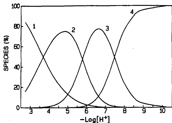
Figure 4. Complex species distribution. Curve 1- \text{Cu}^{2+} . Curve 2- \text{CuL}^{2+} . Curve 3- \text{CuLH}_{-1}^{+} . Curve 4- \text{CuLH}_{-2}
