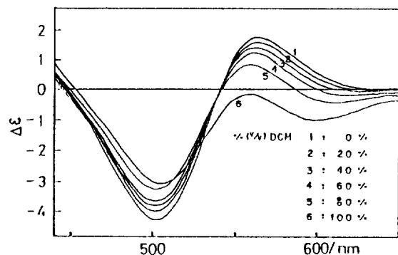
Figure 5. The CD variation of \Delta -[Co(acac) _2 (tn)]ClO _4 as a ratio of dichloromethane(DCM) content in DMSO/DCM mixed solvents.
