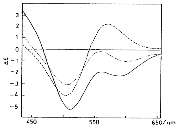
Figure 7. The CD spectra of \Delta -[Co(acac) _2 (tn)]ClO _4 in water(—), dichloromethane(.....), and KBr disc (---)(arbitrary scale).
