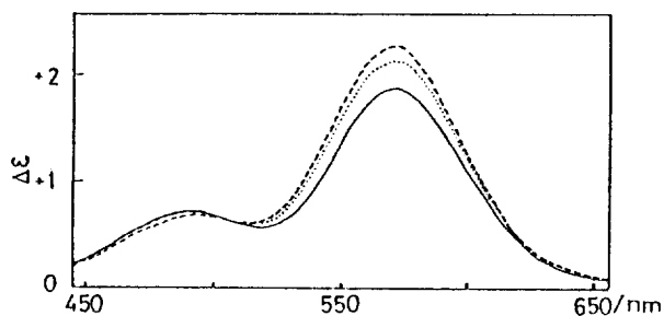
Figure 6. The CD spectra of \Lambda -Na[Co(ox) _2 (en)] in water (—), 80% (v/v) EtOH(.....), and 80%(v/v) acetone(-----).
