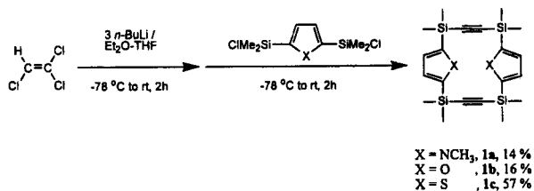
Scheme 1. Syntheses of macrocycles 1a , 1b and 1c .
