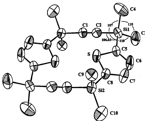
Figure 1. ORTEP view of [\text{C}_{20}\text{H}_{28}\text{S}_2\text{Si}_4] with selected bond lengths (Å) and angles (°): Si(1)-C(2) 1.853(4), Si(1)-C(5) 1.860(6), C(1)-C(2) 1.201(6), C(5)-C(6) 1.364(6), C(6)-C(7) 1.422(10), C(5)-S 1.708(6); C(2)C(1)Si(2) 175.0(5), C(2)Si(1)C(5) 106.0(3), C(2)Si(1)C(3) 110.4(2), C(2)Si(1)C(4) 107.6(2), C(3)Si(1)C(4) 110.8(4), Si(1)C(5)S 122.7(2), Si(1)C(5)C(6) 128.1(5), C(5)C(6)C(7) 112.9(6). Selected dihedral angles (°): C(2)Si(1)C(5)S - 36.84, C(2)Si(1)C(5)C(6) 146.56, C(5)Si(1)C(2)C(1) 52.63, C(8)SC(5)Si(1) - 177.05.
