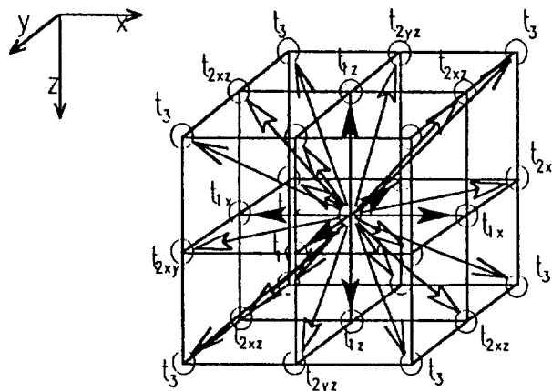
Figure 1. The interaction up to 3rd nearest neighbors. For example, t_x and t_{xy} represent 1st nearest neighbor interaction along x -direction and 2nd one in xy -plane, respectively.
