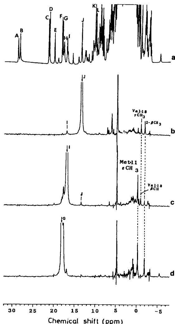
Figure 1. 400 MHz ^1\text{H} NMR spectra of ferricytochrome c_3 from D. vulgaris Hildenborough in 30 mM phosphate buffer ( \text{p}^2\text{H} 7.0) at 30 ^\circ\text{C} . The methyl signals are labeled alphabetically. (a) A normal spectrum. (b-d) NOE difference spectra. The arrows indicate the irradiated positions. The signal at 4.73 ppm comes from \text{H}_2\text{O} . The assignment of the signals is given in the text.
