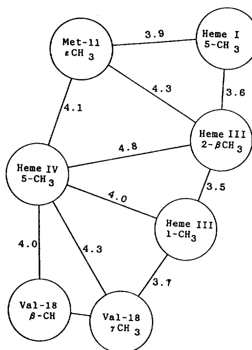
Figure 4. Correlation between the NOE network (solid lines) and the intercarbon distances (Å) in the crystal structure. The assignment is given in the text.
