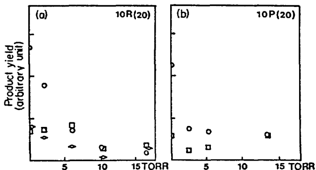
Figure 6. Pressure dependence on the product yields. (a) with 10R(20) laser irradiation. (b) with 10P(20) laser irradiation. ○: 4-Chloro-1-butene. □: 4-Bromo-1-butene. ◇: Butadiene.
