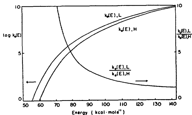
Figure 5. RRKM Calculation of k_a(E) at various energies. k_a(E) , L: k_a(E) for HBr elimination channel. k_a(E) , H: k_a(E) for HCl elimination channel.
