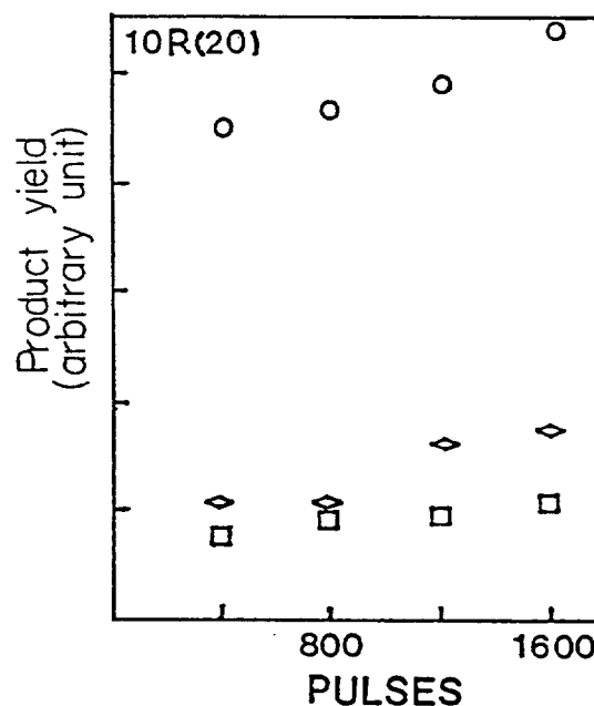
Figure 3. Dependence of the product yields on the number of laser pulses. laser energy: 0.3J. P_{He} = 0 torr. \circ : 4-Chloro-1-butene. \square : 4-Bromo-1-butene. \diamond : Butadiene.
