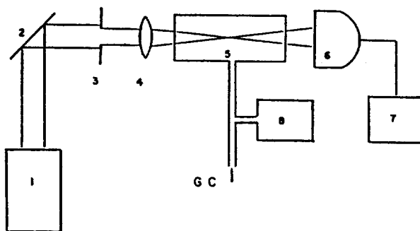
Figure 1. The schematic diagram of IRMPO set up.
