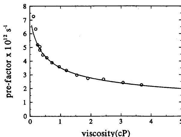
Figure 2. Plot of the reduced isomerization rate vs. the shear viscosity for stilbene in normal alkanes: O experimental results from ref. 1. — present model calculation.
