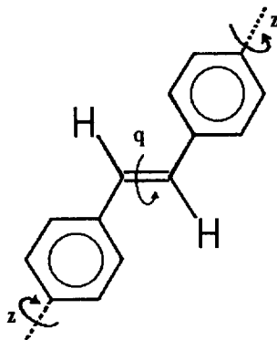
Figure 1. The system coordinates of trans -stilbene.
