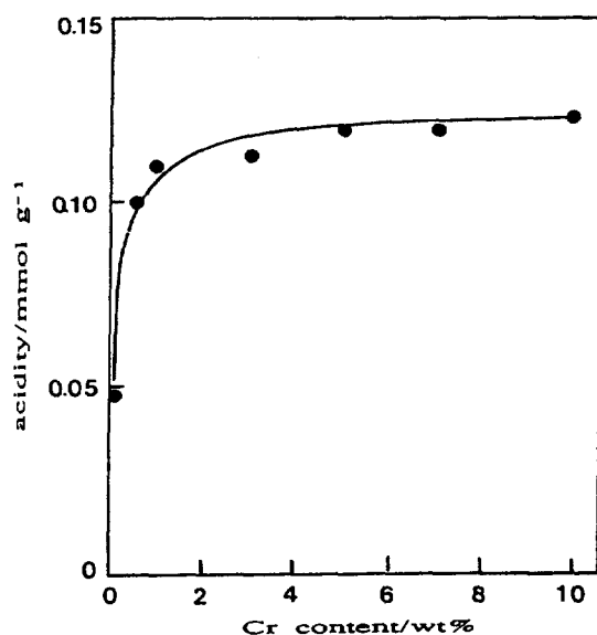
Figure 11. Acidity of CrO x /ZrO 2 against chromium content.
