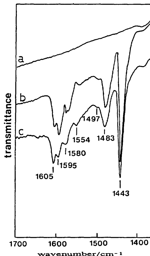
Figure 12. IR Spectra of pyridine adsorbed on 1-CrO x /ZrO 2 : (a) background of 1-CrO x /ZrO 2 after evacuation at 773 K for 1 h; (b) pyridine adsorbed on (a) sample followed by evacuating at room temperature for 1 h; (c) pyridine adsorbed on (a) sample followed by evacuating at 523 K for 1 h.
