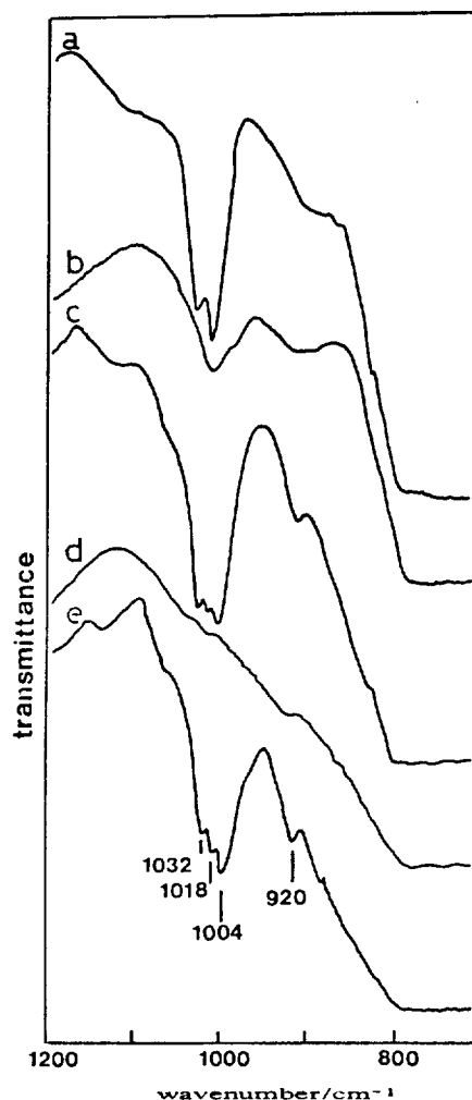
Figure 8. IR spectra of 1-CrO x /ZrO 2 treated under various conditions: (a) after evacuation at 773 K for 1 h; (b) after evacuation at 773 K for 2 h; (c) after oxidation of (b) sample with O 2 (50 torr) at 773 K for 1 h; (d) after reduction of (c) sample with CO (50 torr) at 773 K for 0.5 h; (e) after reoxidation of (d) sample with O 2 (50 torr) at 773 K for 0.5 h.
