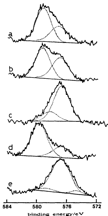
Figure 6. Cr 2p 3/2 fitted for XPS of 3-CrO x /ZrO 2 treated under various conditions: (a) uncalcined sample; (b) sample calcined at 873 K; (c) after reduction of (b) sample with H 2 at 823 K; (d) after reoxidation of (c) sample with O 2 at 823 K; (e) after reaction of (b) sample with n -hexane at 823 K.
