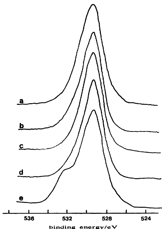
Figure 7. O 1s XPS of 3-CrO x /ZrO 2 treated under various conditions: (a) uncalcined sample; (b) sample calcined at 873 K; (c) after reduction of (b) sample with H 2 at 823 K; (d) after reoxidation of (c) sample with O 2 at 823 K; (e) after reaction of (b) sample with n -hexane at 823 K.
