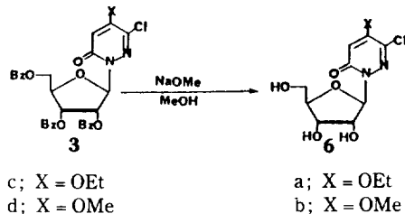
Scheme 3
