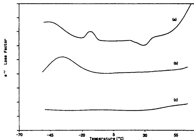
Figure 1. The dielectric loss versus temperature for (a) PL, (b) APL and (c) HTCL at 1 Hz.
