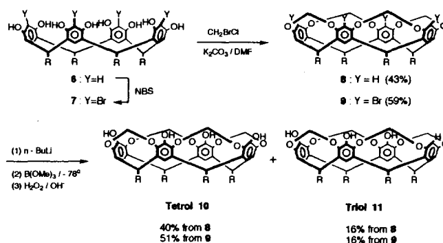
Scheme 1. Synthetic Routes of Tetrol 10 and Triol 11 ( R = (CH_2)_{10}CH_3 ).
