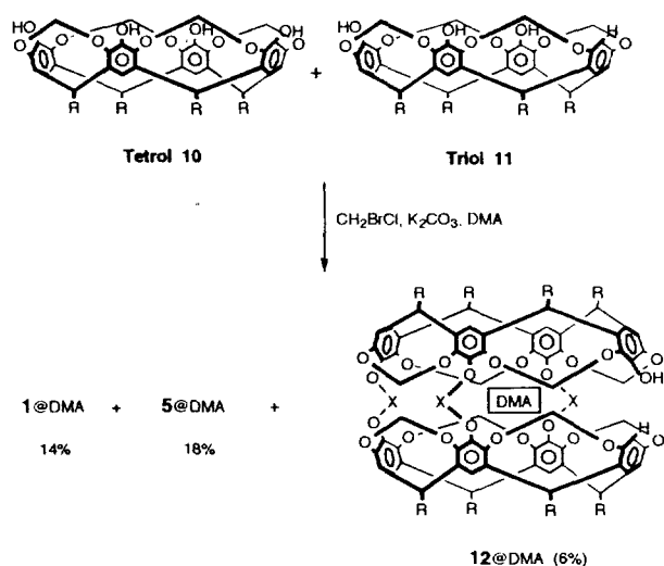
Scheme 2. One-Pot Synthesis of Three Hosts 1 , 5 , and 12 Containing DMA ( \text{R} = (\text{CH}_2)_{10}\text{CH}_3 ).
