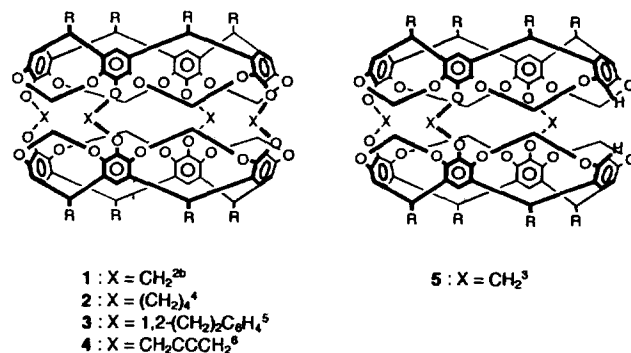
Figure 1. Reported Carcerands and Hemicarcerands.
