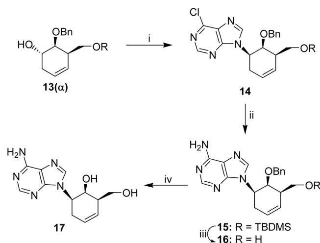
Scheme 3. Reagents: i) 6-chloropurine, DIAD, \text{PPh}_3 , dioxane/DMF; ii) \text{NH}_3/\text{MeOH} , steel bomb; iii) TBAF, THF; iv) Na, \text{NH}_3 /THF, -78^{\circ}\text{C} , 15 min.
