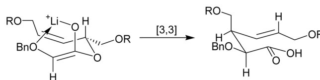
Figure 2. \alpha -chelation controlled [3,3]-sigmatropic rearrangement.
