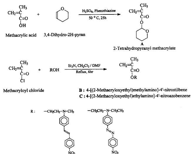
Scheme 1. Monomer syntheses.
