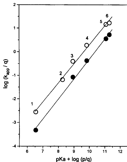
Figure 2. Brønsted-type plots for the aminolysis of p -nitrophenyl phenylacetate (○) and benzoate (●) in H 2 O containing 20 mole % DMSO at 25.0 ± 0.1 °C. The identity of the point is given in Table 2.
