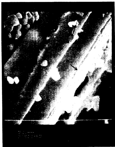
Figure 3. Scanning Electron Micrograph (SEM) of \text{FeMoO}_4\text{Cl} single crystals with board-like morphology ( \times 5000 ). Typical edges of stacked \text{FeMoO}_4\text{Cl} -layers are clearly shown.
