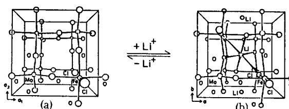
Figure 1. Reversible transition between (a) 2D-tetragonal ( a = 6.672 , b = 5.223 Å) and (b) 3D-monoclinic structure ( a = 7.031 , b = 6.910 , c = 5.040 Å \beta = 91.30^\circ ) 6 upon lithium intercalation.
