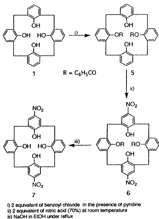
Figure 2. Synthesis of 1,3-Dinitrocalix[4]arene.
