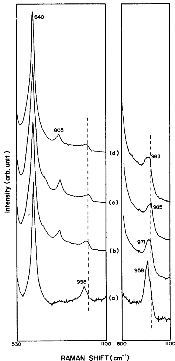
Figure 3. Raman spectra of 10.2 wt% \text{WO}_3 on \text{TiO}_2 , prepared initially at pH 6.8, after drying at 373 K (a) and calcining at 673 (b), 823 (c) and 973 K (d).
