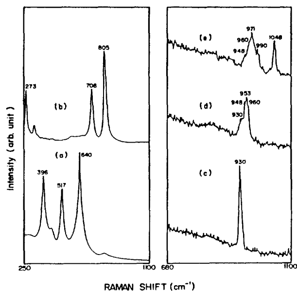
Figure 1. Raman spectra of reference compounds: (a) \text{TiO}_2 (b) \text{WO}_3 and tungstate solutions at pH 11.5 (c) 6.8 (d) and 2 (e).
