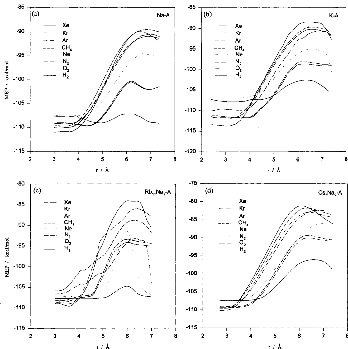
Figure 2. The decapsulation MEPs of some molecules, H_2 , O_2 , N_2 , CH_4 , Ne , Ar , Kr , and Xe , from the \alpha -cage of a) Na-A, b) K-A, c) Rb_{11}Na_1 -A, and d) Cs_3Na_9 -A model zeolite were plotted along the y-axis in Figure 1.
