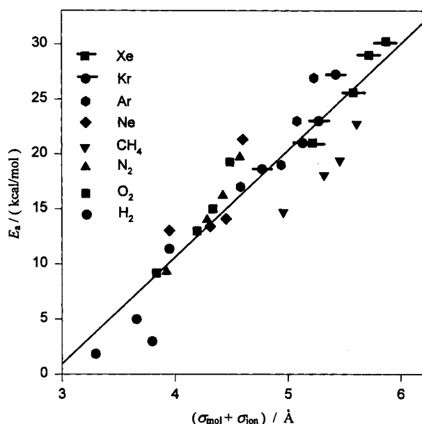
Figure 3. The activation energies, E_a , were plotted against the sum of the kinetic diameters of the encapsulated molecule and of the blocking cation, (\sigma_{\text{mol}} + \sigma_{\text{ion}}) .
