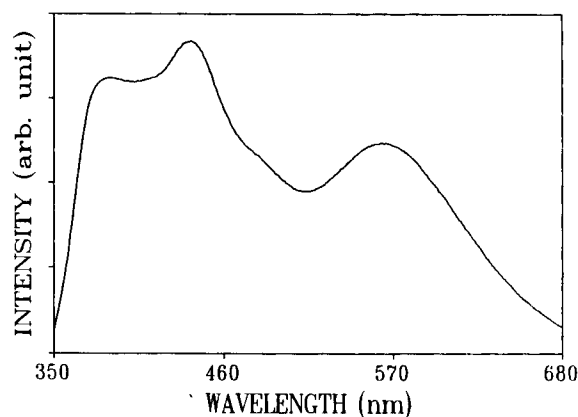
Figure 2. Emission spectrum, excited at 325 nm, of 0.2-mM 6HQN aqueous solution.
