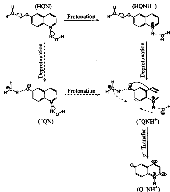
Figure 1. Scheme illustrating the excited state proton and electron transfer mechanism of aqueous 6HQN neutral solution. Protonation to the imine group takes place first, forming HQNH + as the reaction intermediate in the course of protropic tautomerization. (-QNH + ) generated by the subsequent deprotonation of the enol group is transformed into a resonance hybrid structure of quinoid-dominant forms by an intramolecular electron transfer from the deprotonated oxygen atom to the iminium ring.
