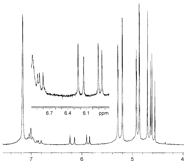
Figure 1. The ^1\text{H} -NMR spectrum of a d_6 -benzene solution of [\text{Pt}(2,6\text{-(Cy}_2\text{PCH}_2)_2\text{C}_6\text{H}_3)(\text{CH}_2=\text{CHCN})]\text{OTf} at ambient temperature in the presence of an excess amount of acrylonitrile shows that the olefinic proton-resonances of the coordinated acrylonitrile appeared at significantly downfield-shifted as compared to those of free acrylonitrile.
