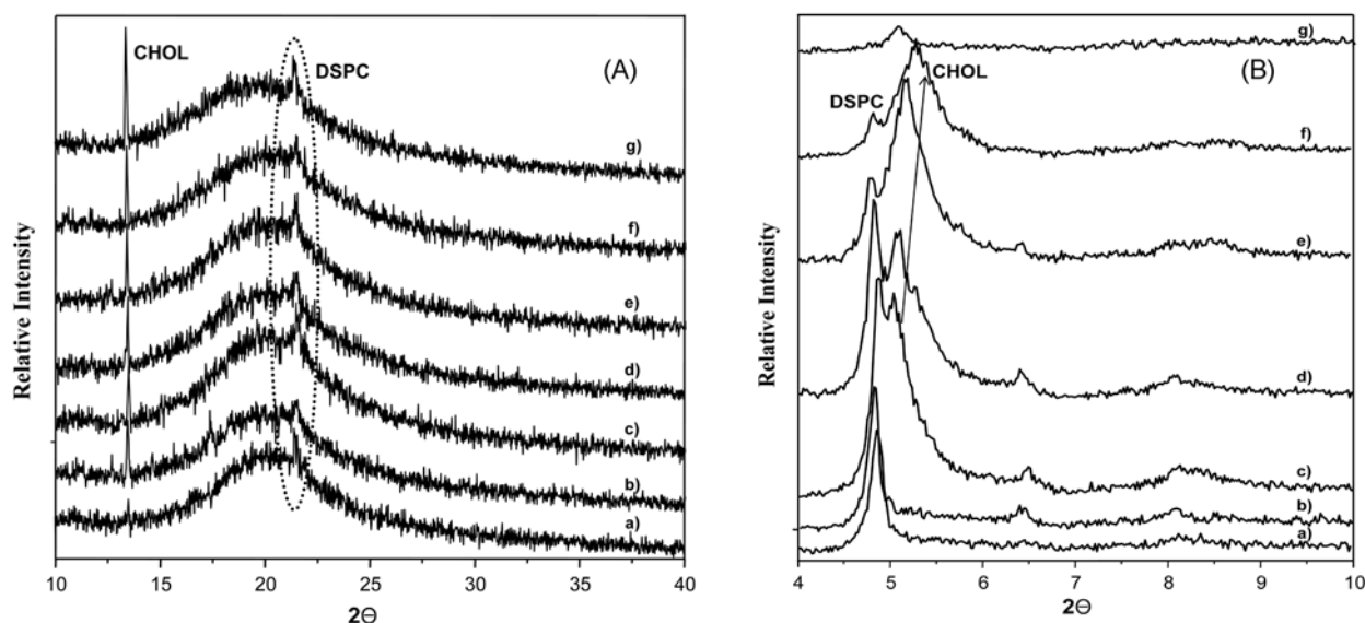
Figure 11. WAXS patterns of DSPC lamellar crystalline phases swollen by an excess of PG depending on the variance of CHOL at 24^\circ\text{C} \pm 1^\circ\text{C} below overall transition temperature ( T_c ): DSPC was fixed at 20.0% w/w and PG was variable correspondingly to increasing the content of CHOL. a) 1.0% w/w CHOL, b) 1.5% w/w CHOL, c) 2.0% w/w CHOL, d) 2.5% w/w CHOL, e) 3.0% w/w CHOL, f) 5.0% w/w CHOL, g) 10.0% w/w CHOL.
