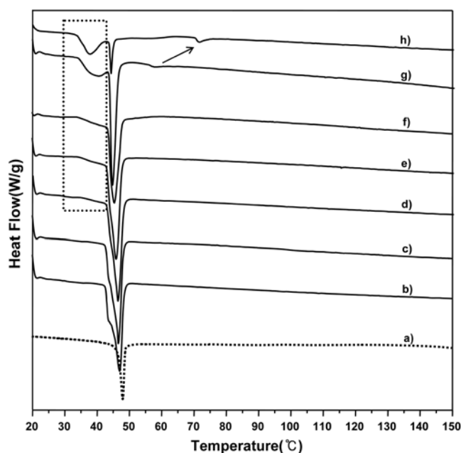
Figure 12. DSC curves of lamellar crystalline phases for each model matrix depending on the variance of CHOL during heating process from 20^\circ\text{C} to 150^\circ\text{C} : DSPC was fixed at 20.0% w/w and PG was variable correspondingly to increasing the content of CHOL.: a) 0% w/w, b) 1.0% w/w, c) 1.5% w/w, d) 2.0% w/w, e) 2.5% w/w, f) 3.0% w/w, g) 5.0% w/w, h) 10.0% w/w.
