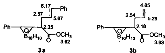
Figure 1. ^1\text{H} NMR assignment of C-allylated carboranyl acetic ester.
