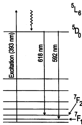
Figure 1. Schematic energy levels of aqueous Eu 3+ to show the employed transitions for excitation and emission.
