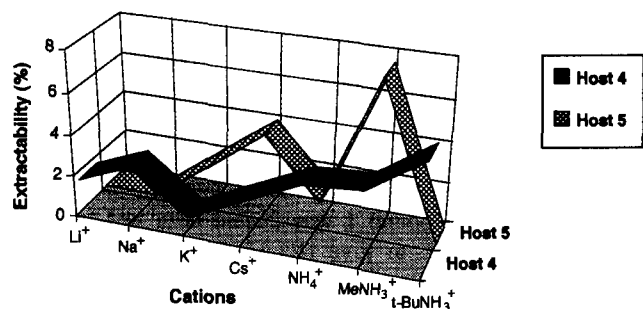
Figure 2. Liquid-liquid Extractability Spectra of Calix[4]crown 4 and 5 8a of Alkali Metal and Alkylammonium Picrates ( [H]=3.0 \times 10^{-3} M, [GPic]=6.0 \times 10^{-5} M, [GCl]=0.5 M, Average Values of Two Trials).
