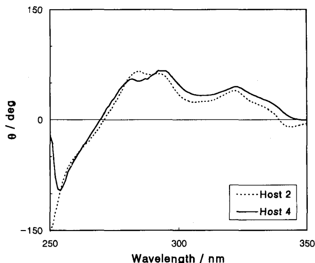
Figure 1. CD Spectra of Host 2 and 4 at 25 °C ([ 2 ]=[ 4 ]= 1.0 \times 10^{-4} M in CH 2 Cl 2 ).
