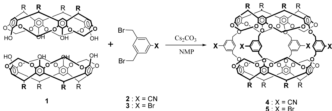
Scheme 1. Synthesis of 4-directionally functionalized hemicarcerands 4 and 5 (R = Heptyl).
