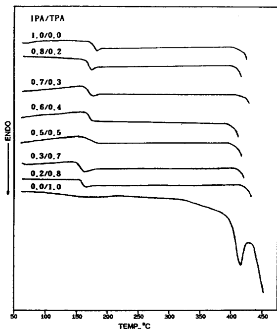
Figure 4. DSC thermograms of the polymers ( N_2 atmosphere, heating rate; 10^\circ C/min ).
