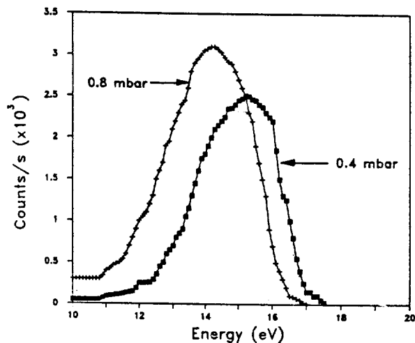
Figure 8. ^{55}\text{Mn}^+ ion intensity as a function of the ion energy window at 15 V bias voltage and 0.4 and 0.8 mbar pressure, respectively.
