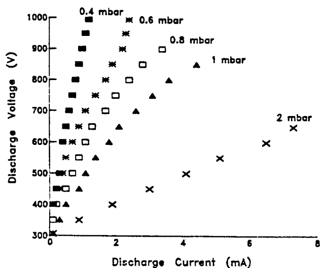
Figure 4. Characteristic voltage/current showing the effect of pressure on the glow discharge.
