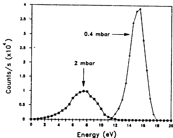
Figure 9. ^{40}\text{Ar}^+ ion intensity as a function of the ion energy window at 15 V bias voltage, and at 0.4 and 2 mbar pressures, respectively.
