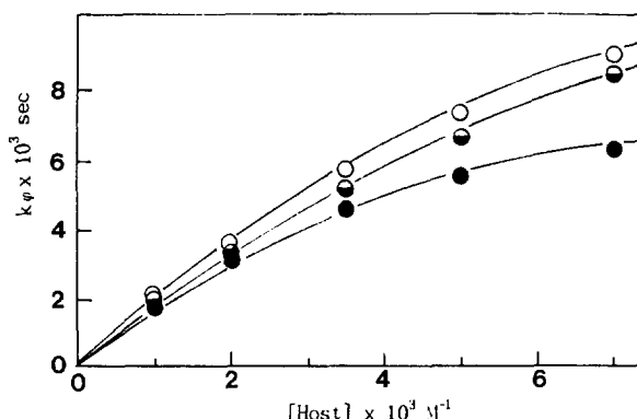
Figure 1. Dependence of apparent first-order rate constant ( k_o ) for the cleavage of p -nitrophenyl ( R )- \alpha -methoxyphenylacetate on [host]. Hosts are CD-S-PG (●), \beta -CD (◐), and CD-R-PG (○).
