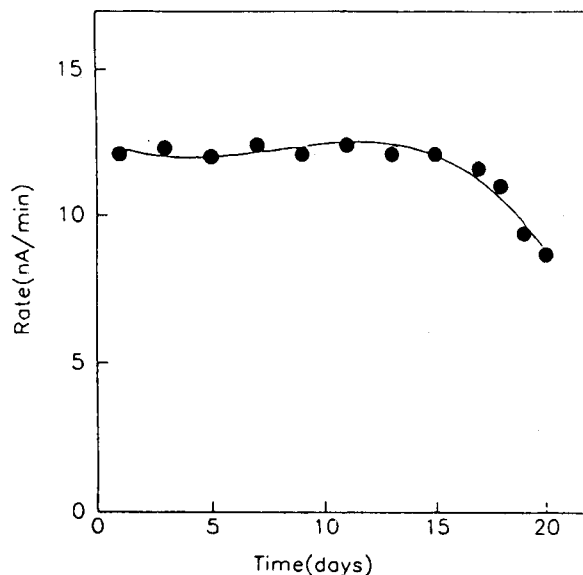
Figure 5. Life time of the immobilized coupled enzyme membrane (30 \mu\text{L} of 1,000 units/mL of urease and 20 \mu\text{L} of 1,000 units/mL of GL-DH).
