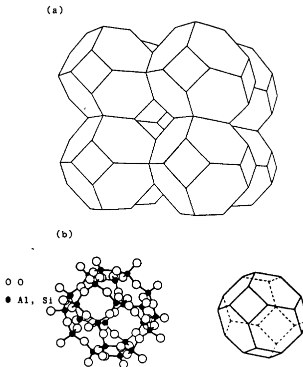
Figure 1. (a) The stacking of 14-hedra of sodalite structure, (b) Sodalite unit.
